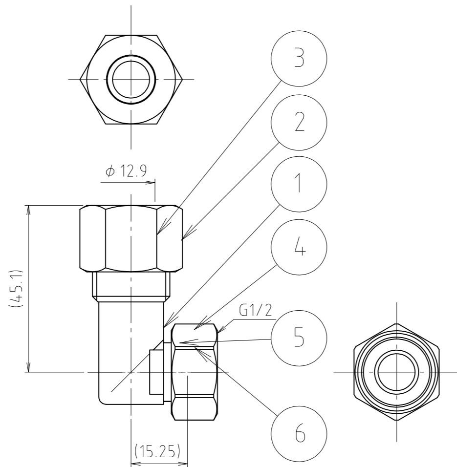
G1/2×12.7
